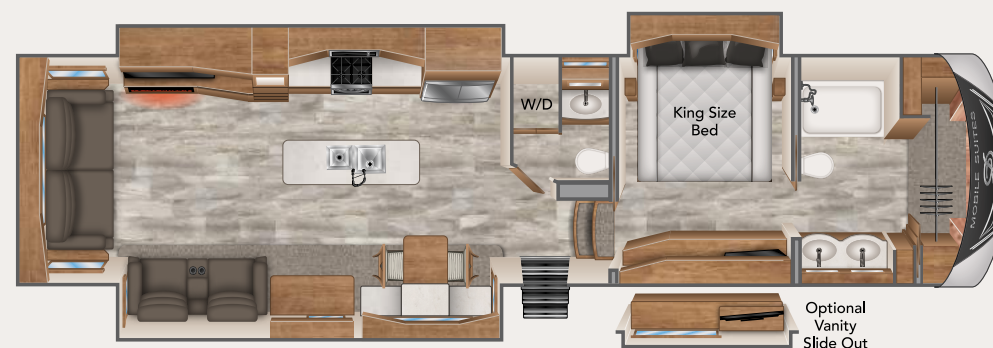
44 HOUSTON Length 44' 2" | Est. Dry 20,300
